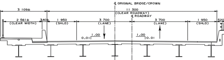
Figure 1. Final lane configuration of the Gordon E. Taylor Bridge
